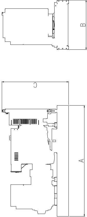
Open set
