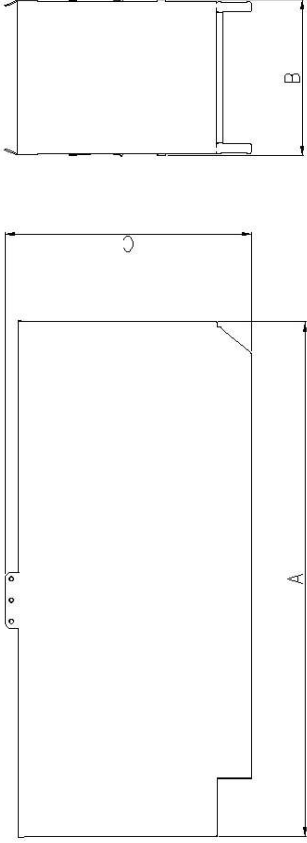
Enclosed set
